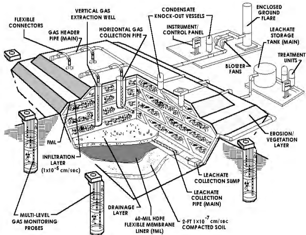
Figure 1. Landfill Components 10
